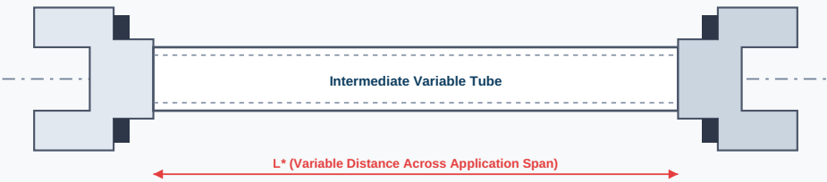
Figure 1: Sectional technical architecture of the CENTAFLEX-E Type 3-GZ bridging configuration.
